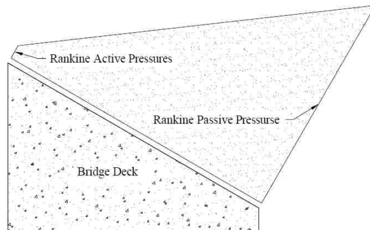
Figure 2-9: Nonuniform lateral pressure distribution, adapted from Sandford and Elgaaly (1993)
