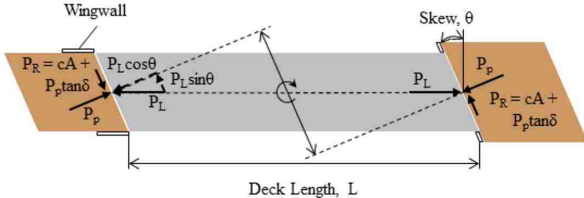
Figure 2-10: Typical forces on a skewed bridge from lateral loading (Franke 2013)
